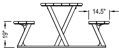
SIDE ELEVATION
